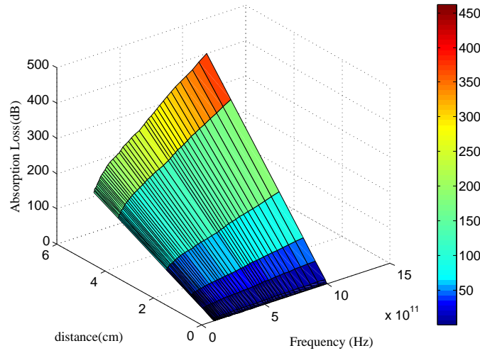
FIG. 62: Absorption Loss at Different Distances for Water.
