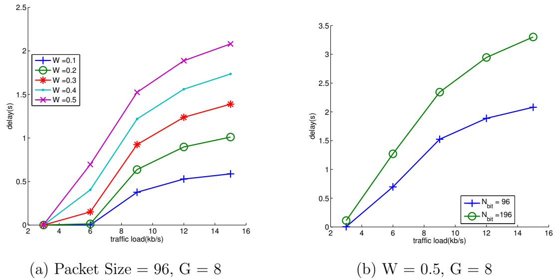
FIG. 20: Average Delay.
